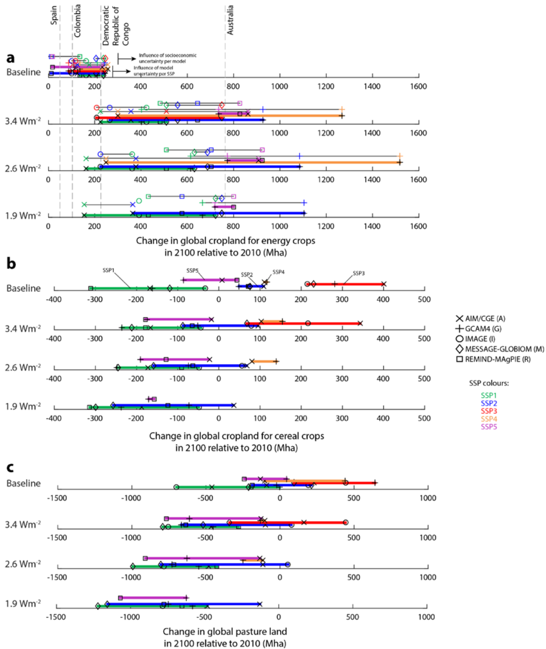
Supplementary Figure 19 | Variation of change of land area dedicated to specific uses in 2100 relative to 2010.
