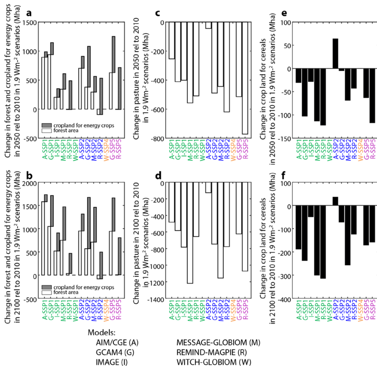
Supplementary Figure 18 | Change of land area in 2050 and 2100 relative to 2010 levels. Global land area change for forest, cropland for energy crops (panels a and b ), land for pasture (panels c and d ), and land for cereals (panels e and f ) is shown.
