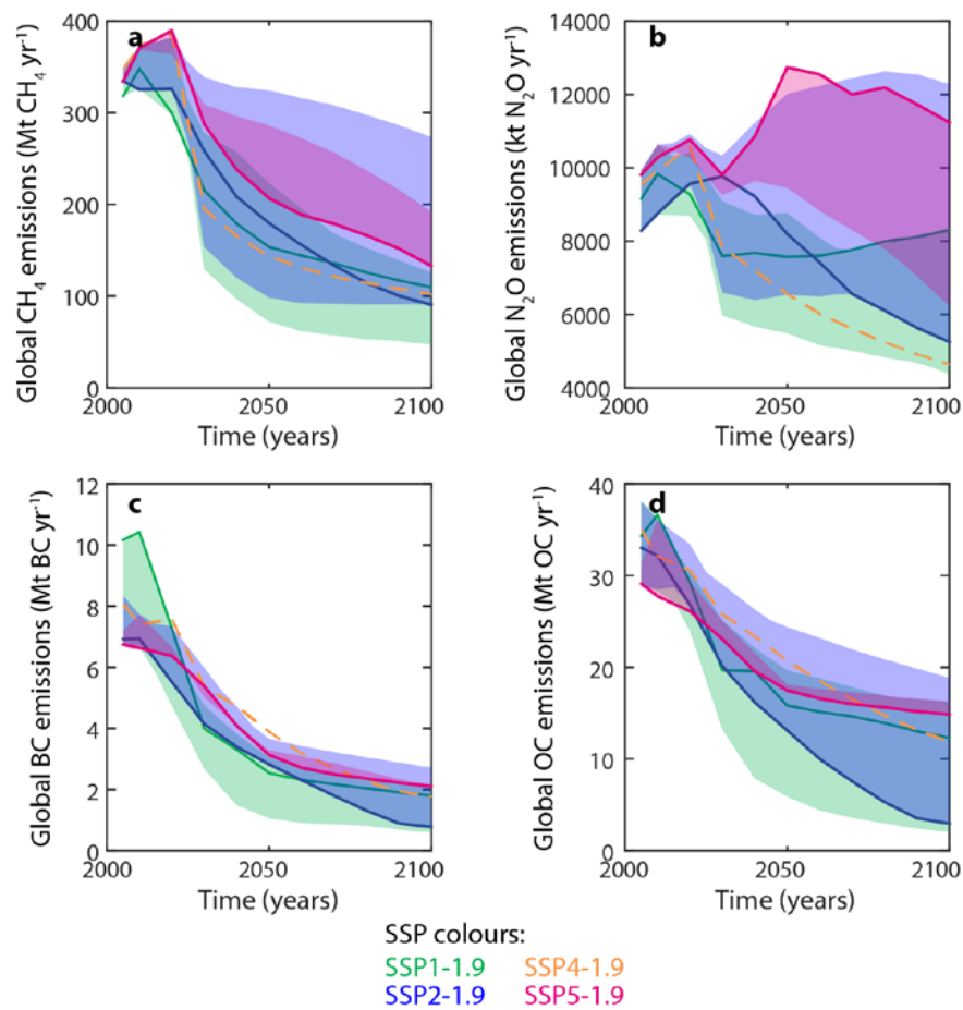
Supplementary Figure 3 | Evolution of anthropogenic emission of greenhouse gases and aerosols in 1.9 \text{ Wm}^{-2} scenarios. a , global total \text{CH}_4 emissions; b , global total \text{N}_2\text{O} emissions; c , global black carbon (BC) emissions; d , global organic carbon (OC) emissions. Shaded areas show the range per SSP, solid lines the marker scenarios for each SSP, and dashed lines are used in case only one scenario was available for a particular SSP and this scenarios was not the marker implementation of that SSP.
