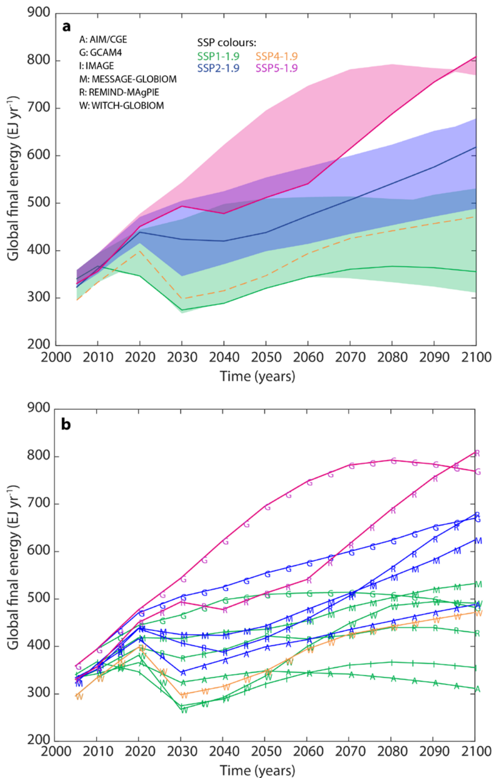
Supplementary Figure 11 | Final energy demand in 1.9 Wm -2 scenarios. a , Shaded areas show the range per SSP, solid lines the marker scenarios for each SSP, and dashed lines are used in case only one scenario was available for a particular SSP and this scenario was not the marker implementation of that SSP; b , as panel a , but with single models highlighted.
