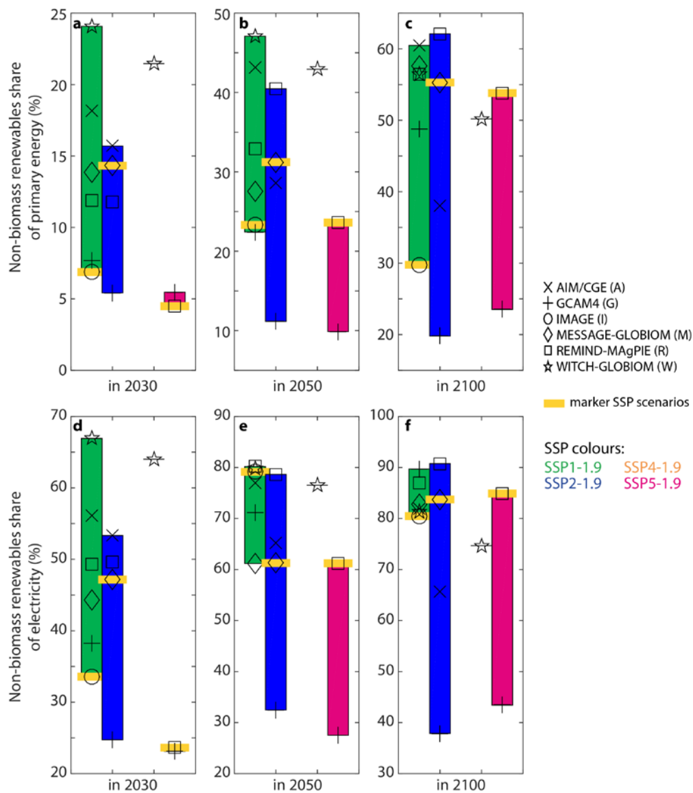
Supplementary Figure 12 | Non-biomass renewable energy share of primary energy and of electricity in 1.9 Wm -2 scenarios. Panels a , b , and c show values for 2030, 2050, and 2100, respectively, for primary energy (direct equivalent accounting); Panels d , e , and f show values for 2030, 2050, and 2100, respectively, for the share of non-biomass renewables of electricity (i.e. secondary energy). Non-biomass renewables encompass solar, wind, hydro, and geothermal energy.
