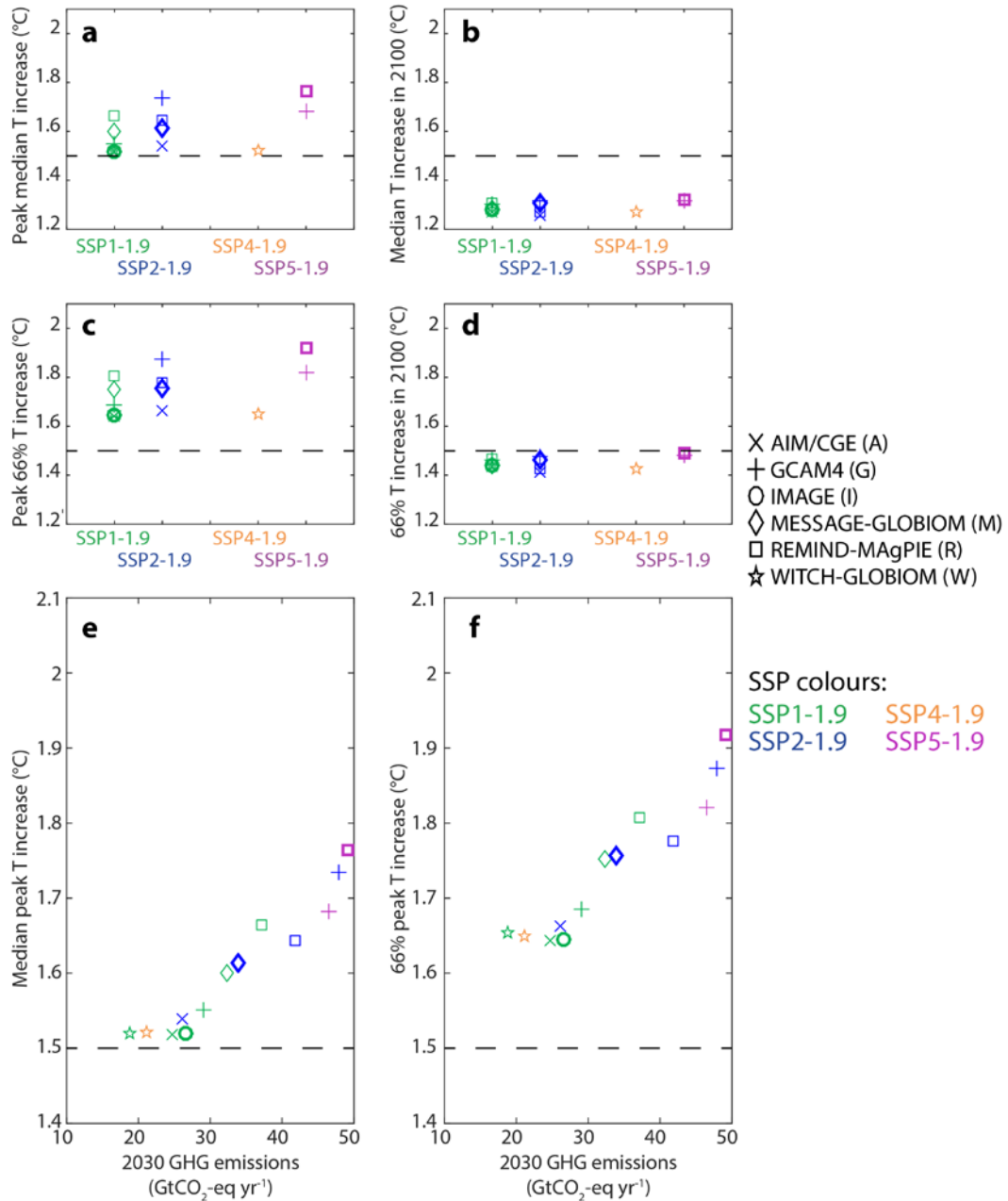
Supplementary Figure 8 | Temperature outcomes of 1.9 Wm -2 scenarios. Distribution of median peak (panel a ) and year-2100 (panel b ) global mean temperature increase relative to preindustrial levels computed with the reduced complexity carbon-cycle and climate model MAGICC 46 in a probabilistic setup 46,47 ; c,d , as panels a and b but for 66 th percentile warming; e,f , correlation between 2030 global GHG emissions levels and peak temperature increase. Bold symbols show the marker implementation of each SSP.
