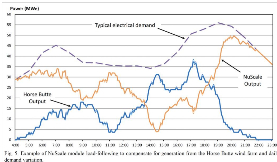
Fig. 5. Example of NuScale module load-following to compensate for generation from the Horse Butte wind farm and daily demand variation.
